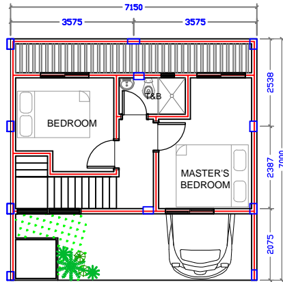
SECOND FLOOR PLAN SCALE: 1:150 METERS
