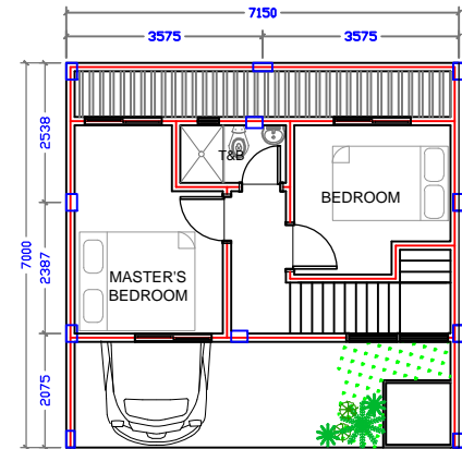
SECOND FLOOR PLAN SCALE: 1:150 METERS
