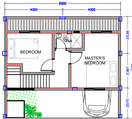
SECOND FLOOR PLAN SCALE: 1:150 METERS
