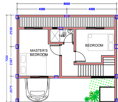
SECOND FLOOR PLAN SCALE: 1:150 METERS
