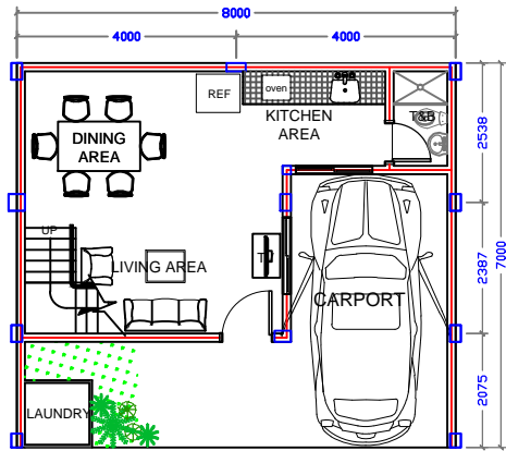
GROUND FLOOR PLAN SCALE: 1:150 METERS
