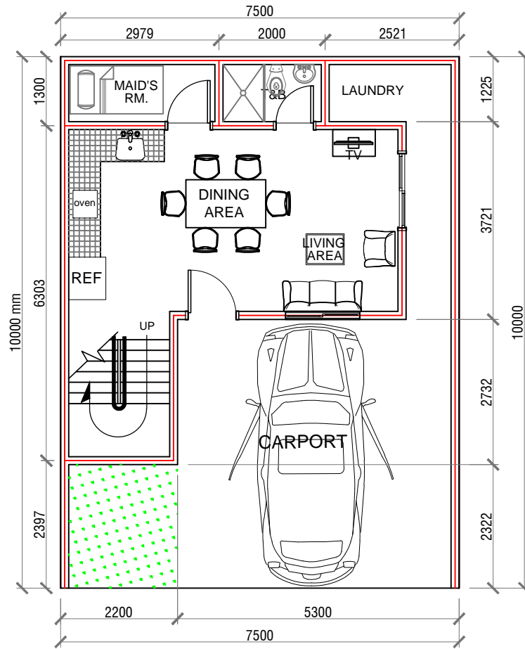
TYPICAL GROUND FLOOR PLAN SCALE: 1:100 METERS
