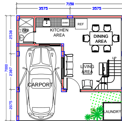
GROUND FLOOR PLAN SCALE: 1:150 METERS
