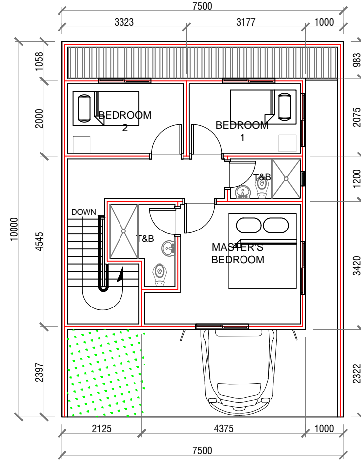
TYPICAL SECOND FLOOR PLAN SCALE: 1:100 METERS
